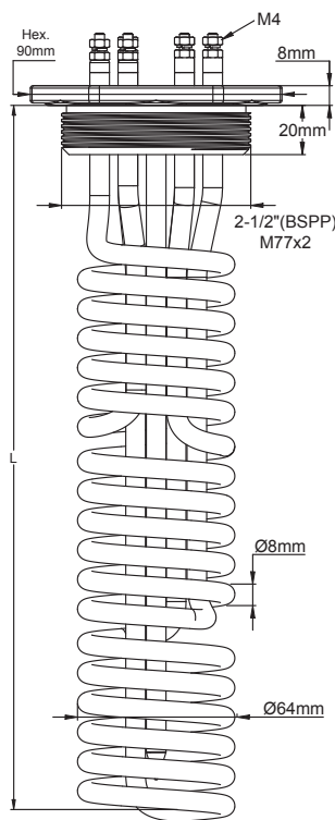
With 2½" BSPP and M77x2 fittings
