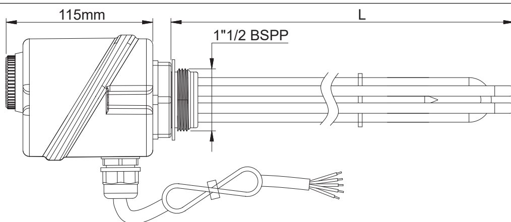
3 Poles 400V heater
