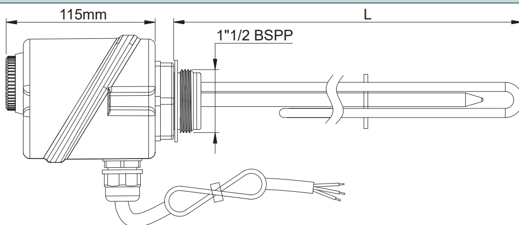
Single pole 230V heater
